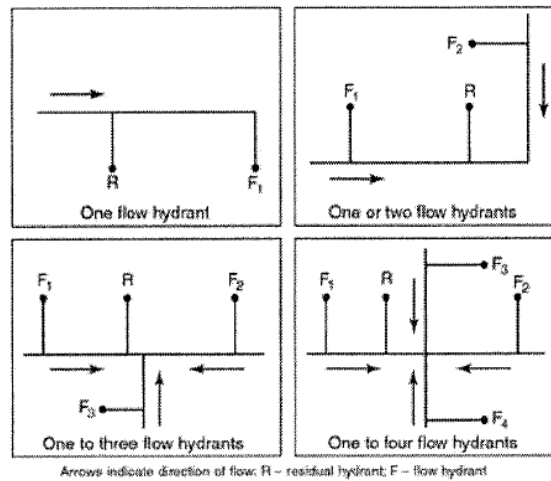
FIGURE 4.3.4 Suggested Test Layout for Hydrants.
