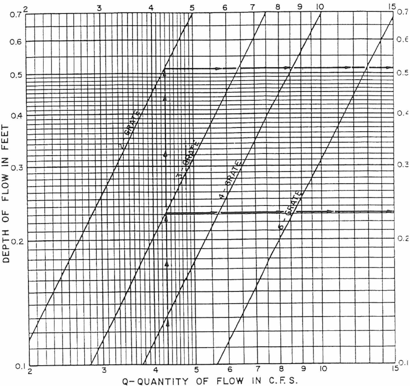
GRATE INLET CAPACITY CURVES AT LOW POINT
