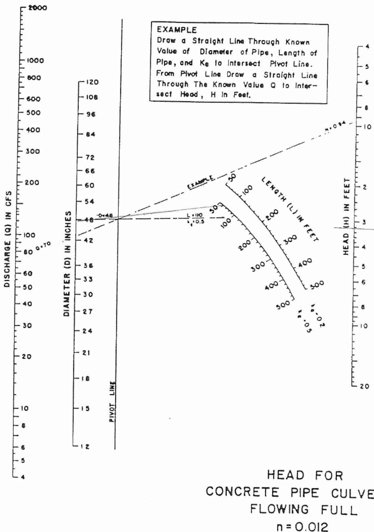
FIGURE 3.26: HEAD FOR CONCRETE PIPE CULVERTS FLOWING FULL
