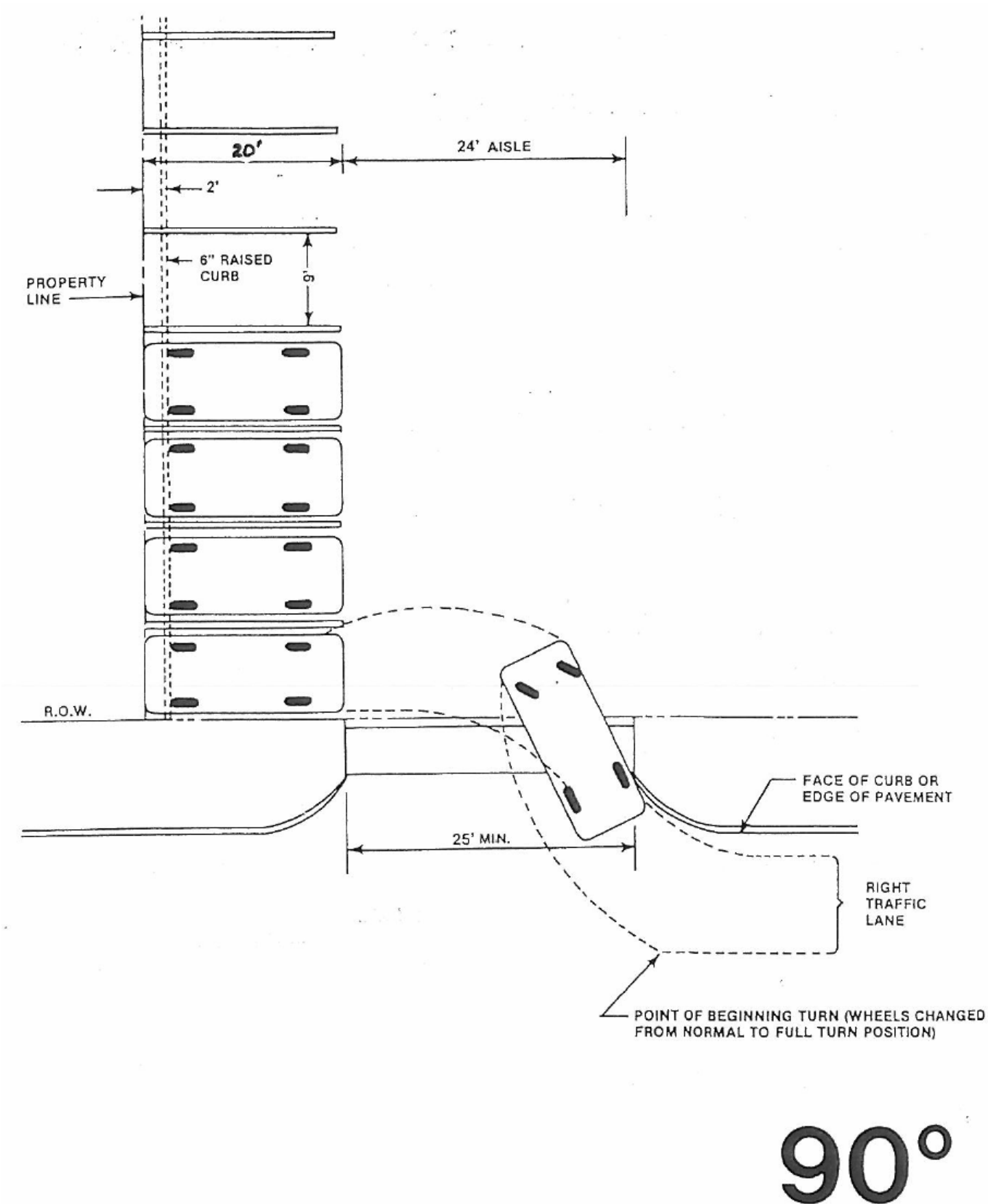
FIGURE 2.8: 90° PARKING (SINGLE ROW)
