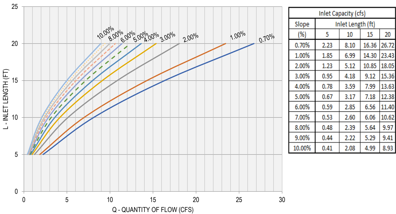
FIGURE 3.8: CURB INLET CAPACITY ON-GRADE LOCAL RESIDENTIAL STREET
