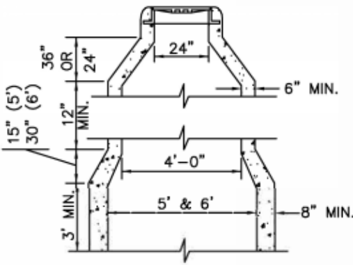
TRANSITION DETAIL FOR 5' & 6' DIA. M.H.'S N.T.S.
