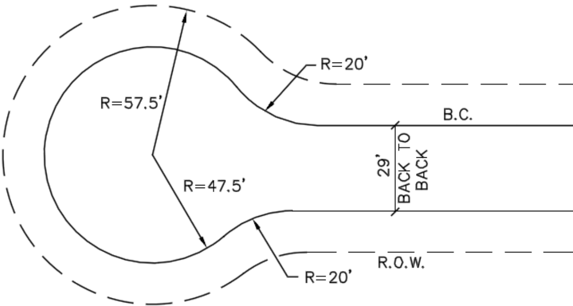
TYPICAL CUL-DE-SAC
