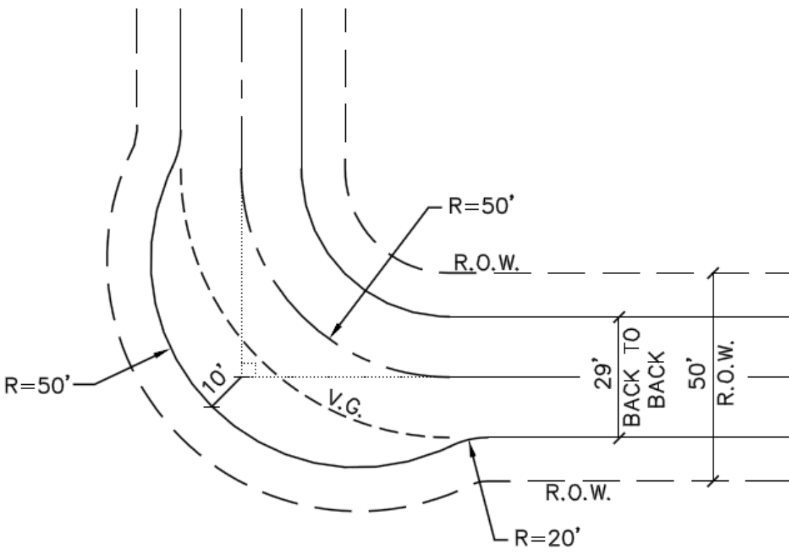
TYPICAL EYEBROW
