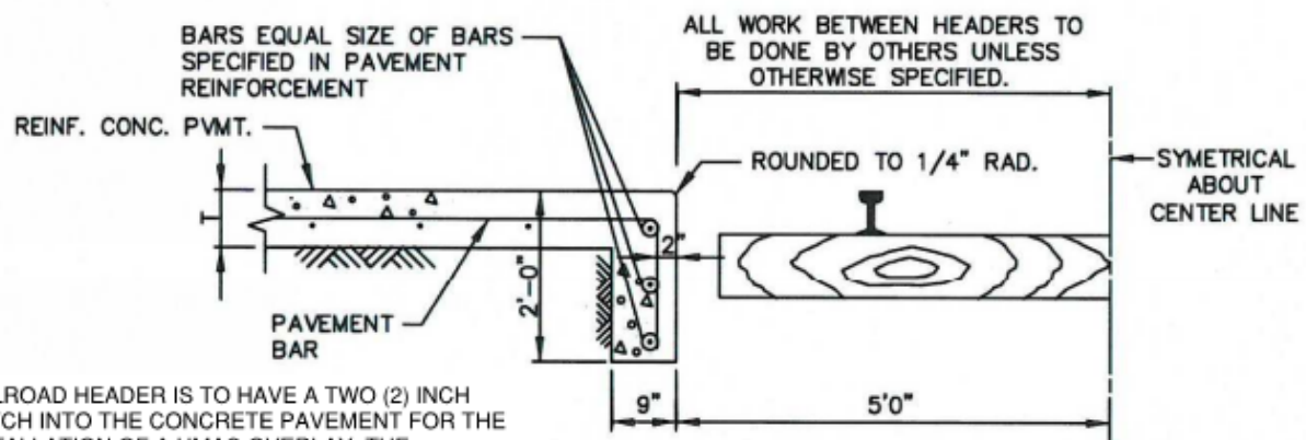
STREET HEADER AT RAILROAD N.T.S.
