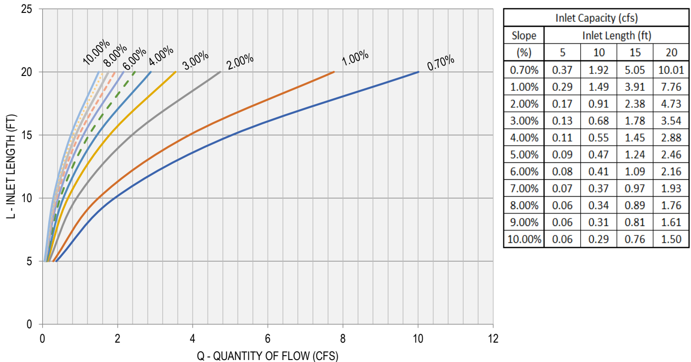
FIGURE 3.9: CURB INLET CAPACITY ON-GRADE ALLEY
