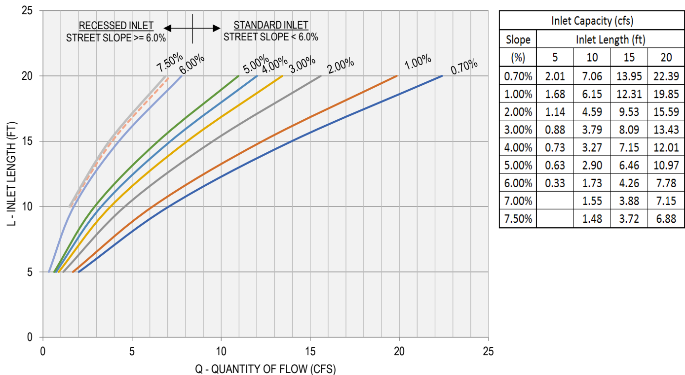
FIGURE 3.7: CURB INLET CAPACITY ON-GRADE MINOR COLLECTOR
