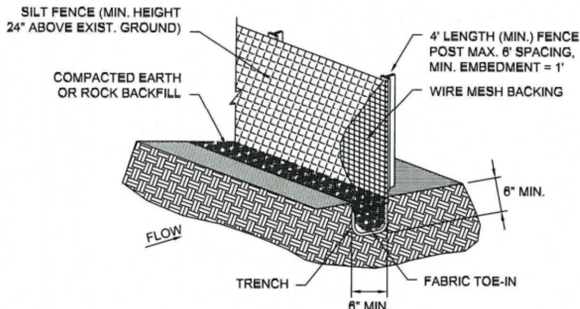
SILT FENCE
