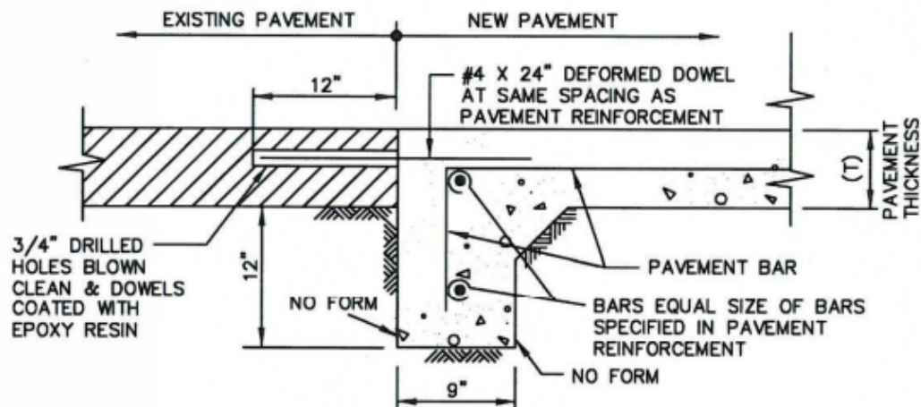
STREET HEADER AT EXISTING PAVEMENT N.T.S.
