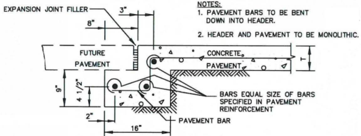
STREET HEADER FOR FUTURE PAVEMENT N.T.S.
