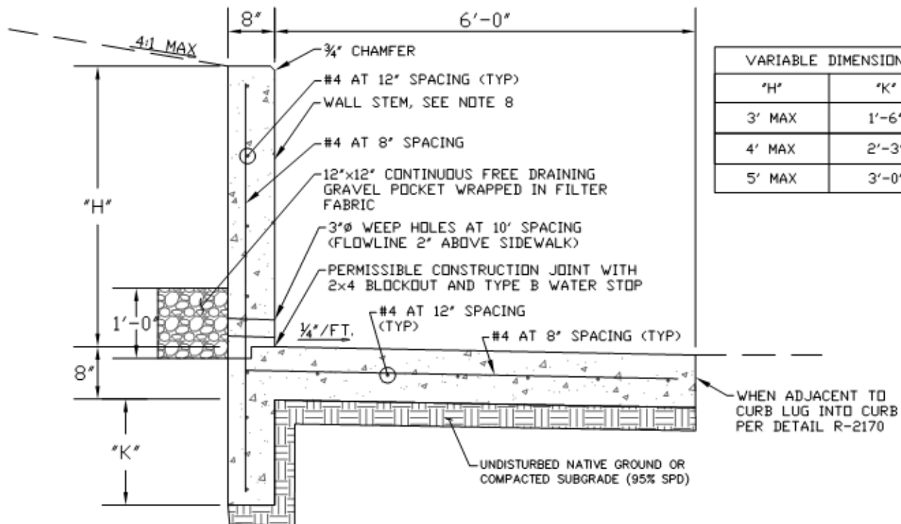
RETAINING WALL WITH INTEGRAL SIDEWALK
