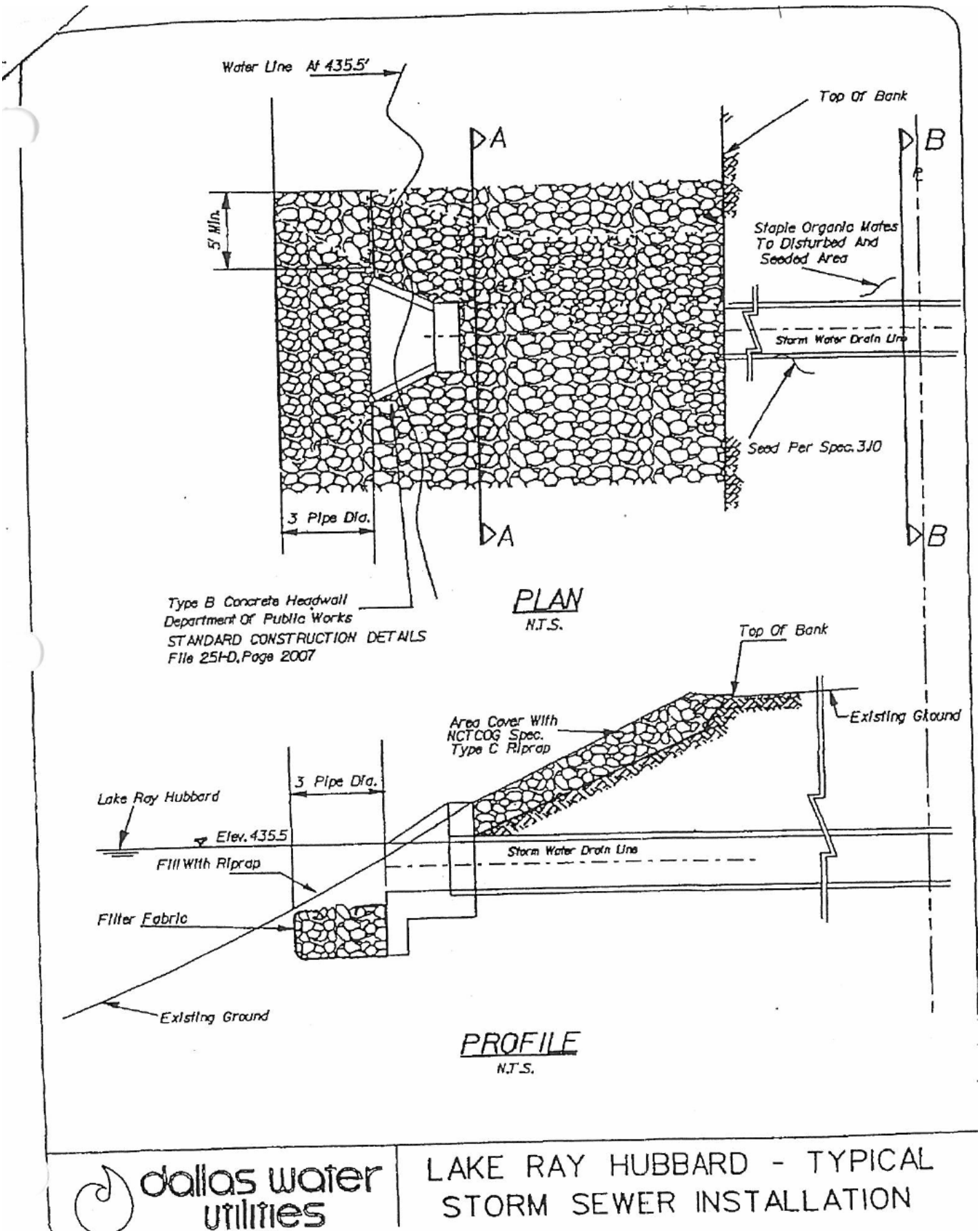
FIGURE 3.22: LAKE RAY HUBBARD TYPICAL STORM SEWER INSTALLATION
