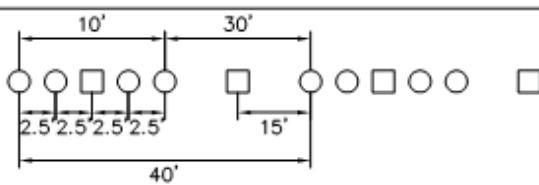
BROKEN WHITE LANE LINE
