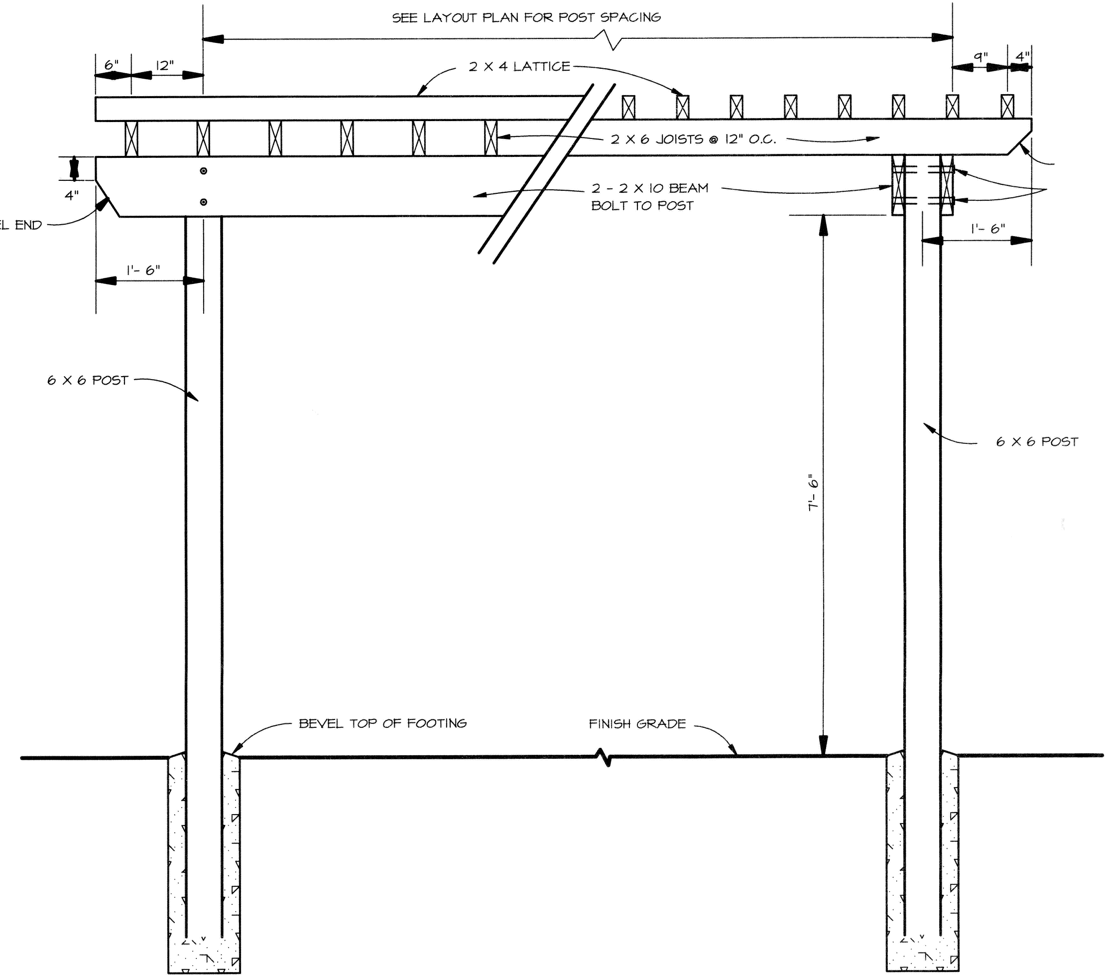
1 SHADE STRUCTURE DETAIL L4
