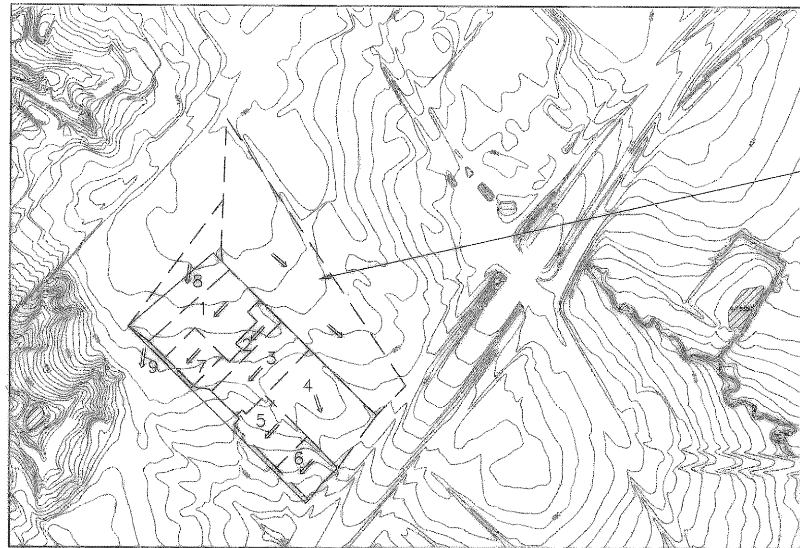
OFFSITE DRAINAGE
