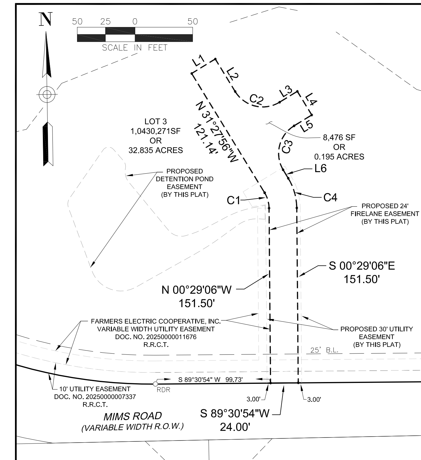
FIRELANE EASEMENT
