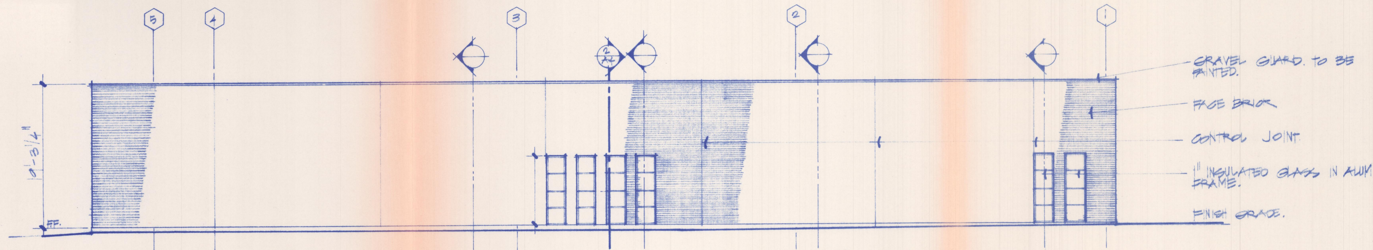
1 north elevation 1/8" = 1'-0"
