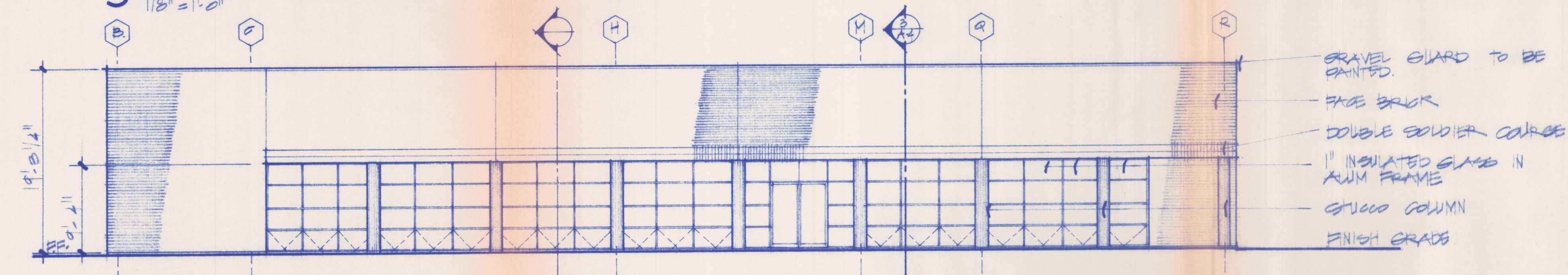
4 west elevation 1/8" = 1'-0"
