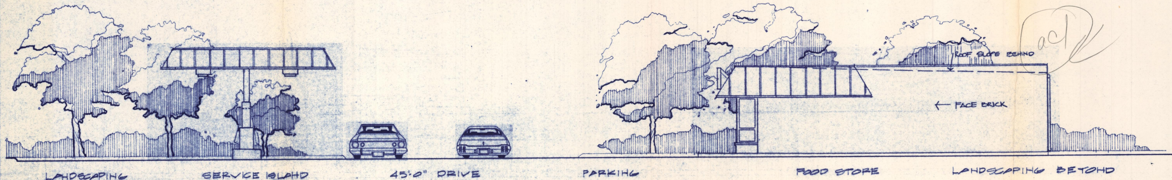
07 West Elevation 1/8" = 1'-0"
