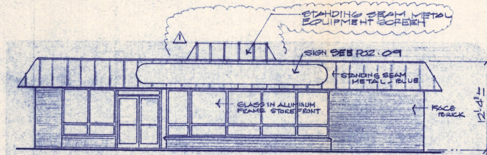
03 North Elevation
