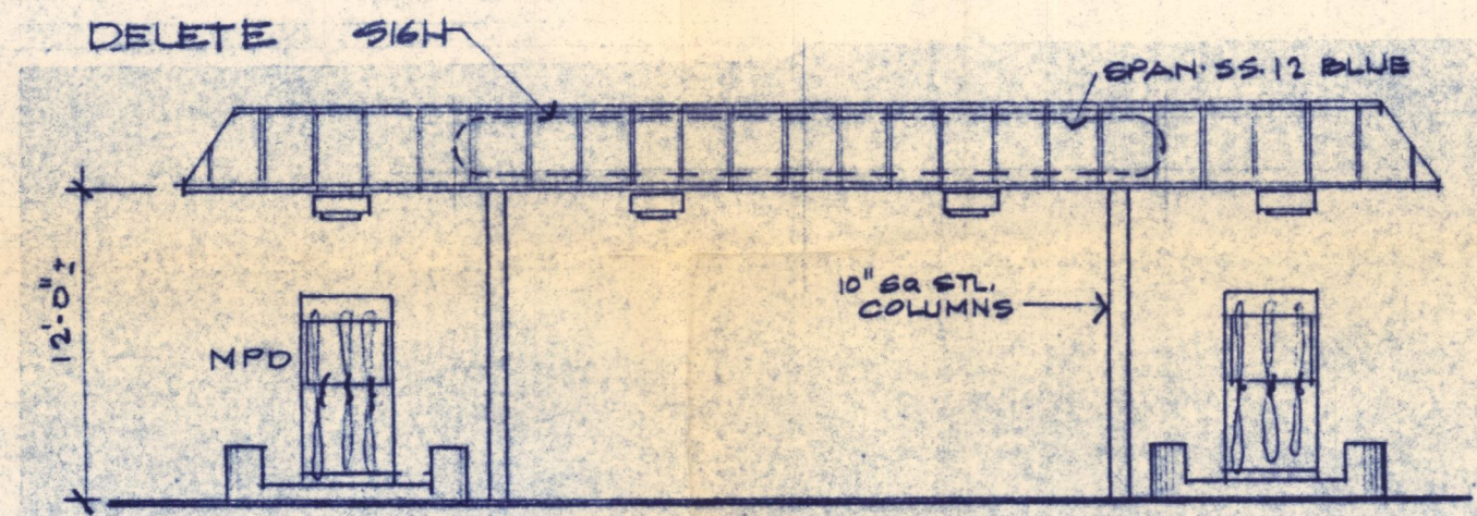
08 Canopy North 1/8" = 1'-0"
