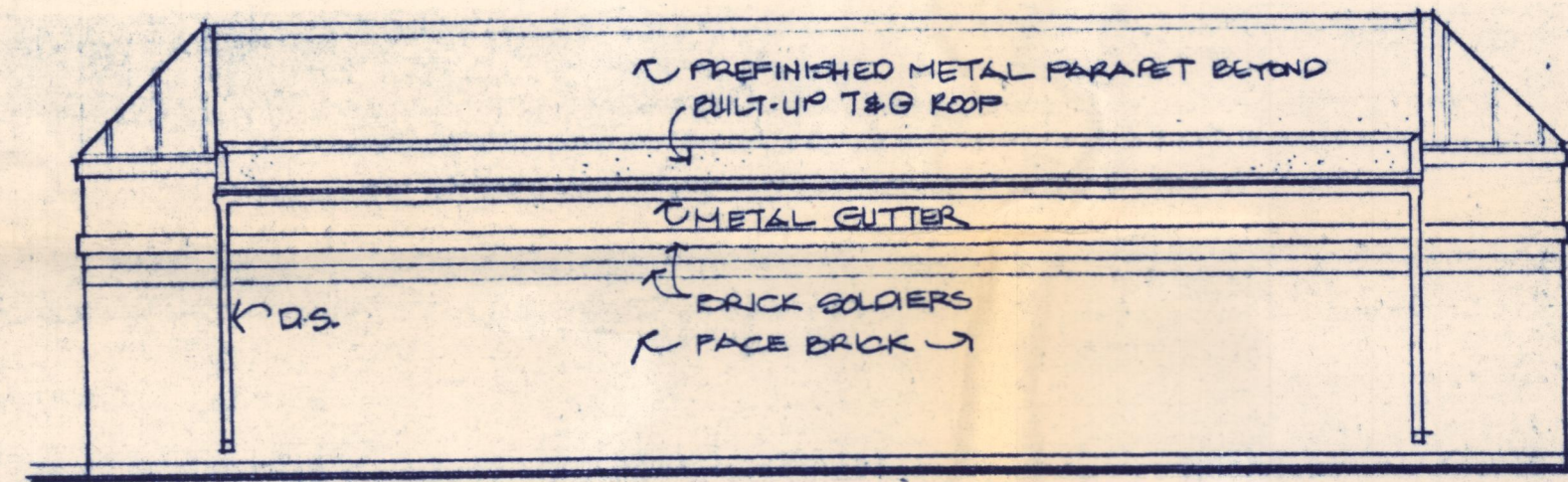
02 South Elevation 1/8" = 1'-0"
