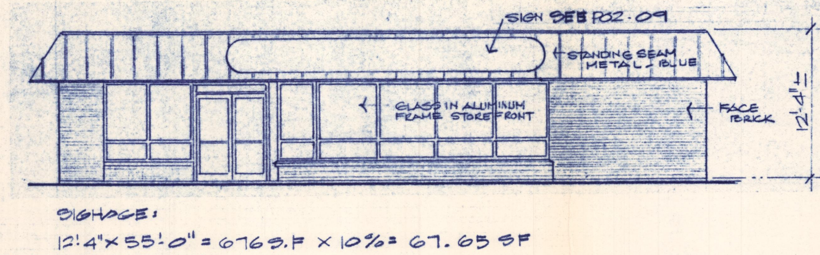
03 North Elevation 1/8" = 1'-0"
