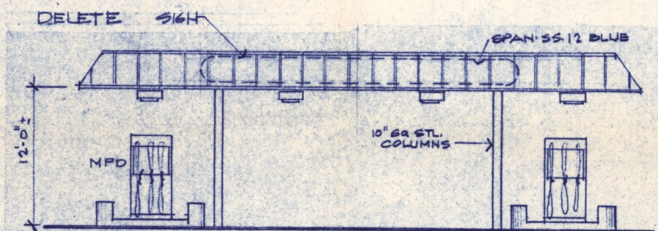
08 Canopy North
