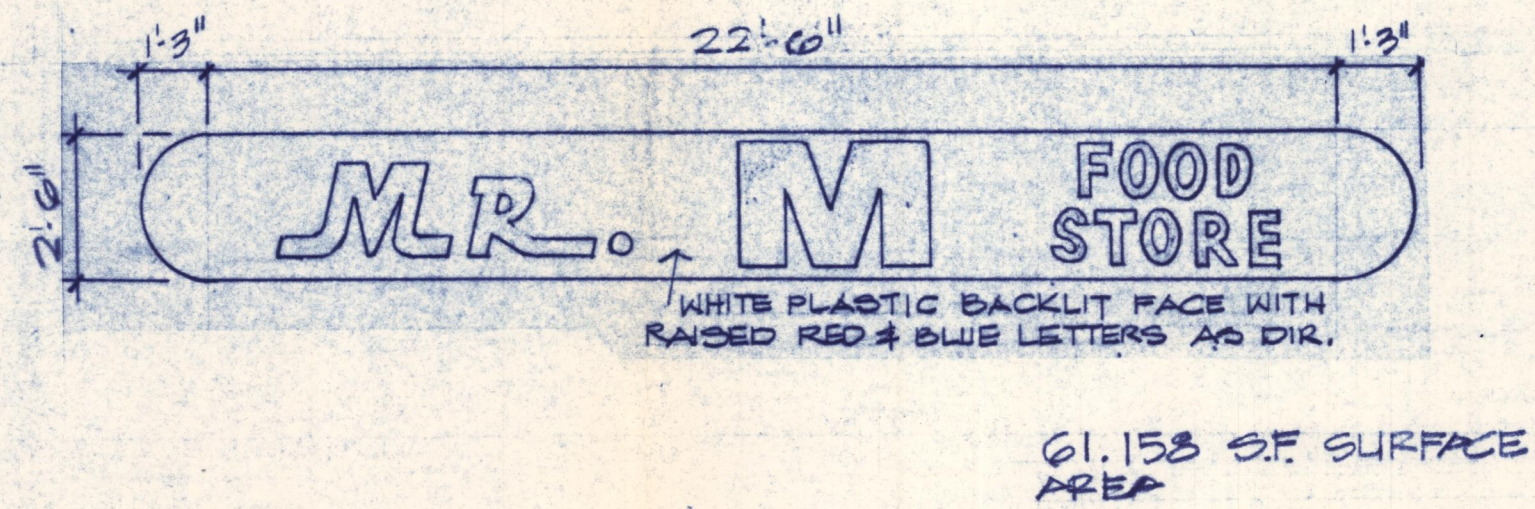
09 Sign Detail 1/4" = 1'-0"
