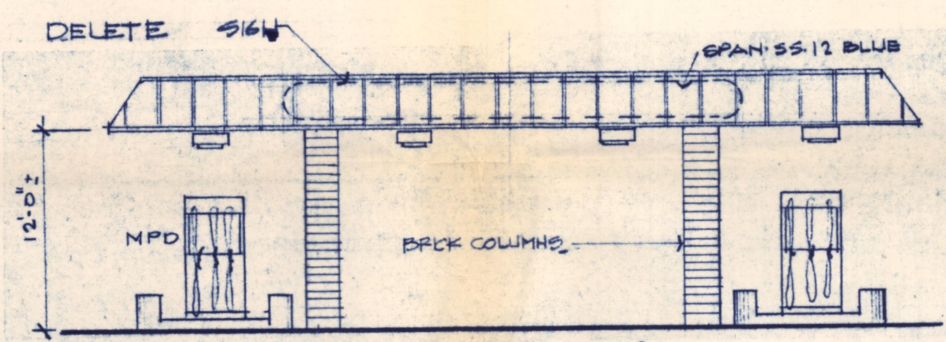
08 Canopy North 1/8" = 1'-0"
