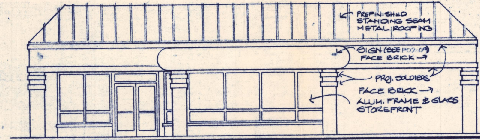
03 North Elevation 1/8" = 1'-0"
