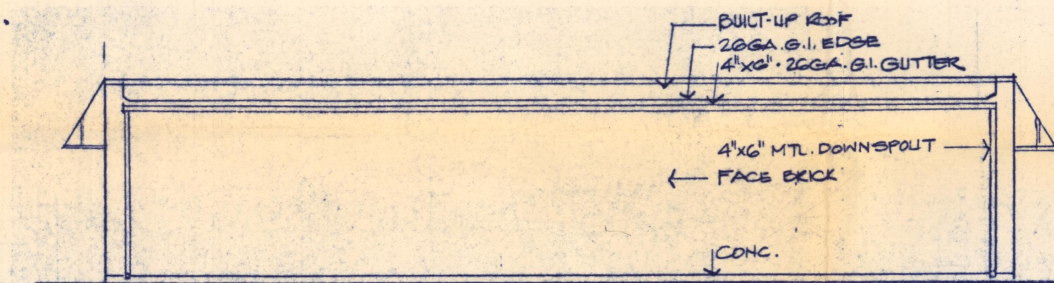
02 South Elevation 1/8" = 1'-0"
