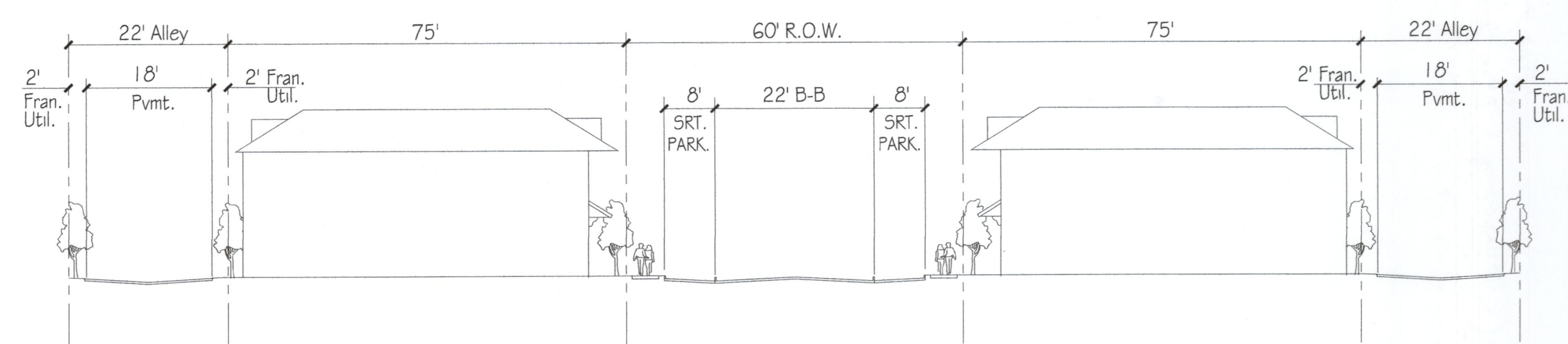
Tract 3 - TH - Typical Section n.t.s.
